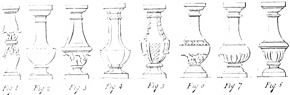
NO. 59. PLAIN AND ENRILED BALUSTERS. ROUND, SQUARE, AND OCTAGONAL ON PLAN.
